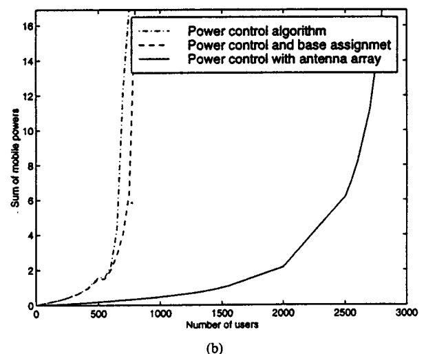
Fig. 6. (a) Total mobile powers versus the iteration number. (b) Total mobile powers versus the number of users.
