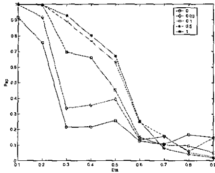
Fig. 4. P_{sp} vs. \eta in a WS small-world network
