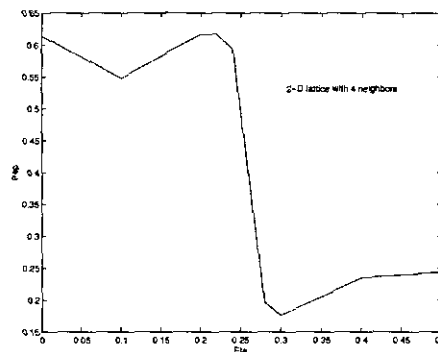
Fig. 3. P_{sp} vs. \eta in a 2-D lattice
