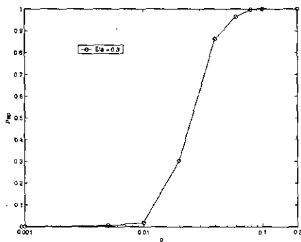
Fig. 2. P_{sp} vs. p in random graphs with \eta fixed at 0.3
