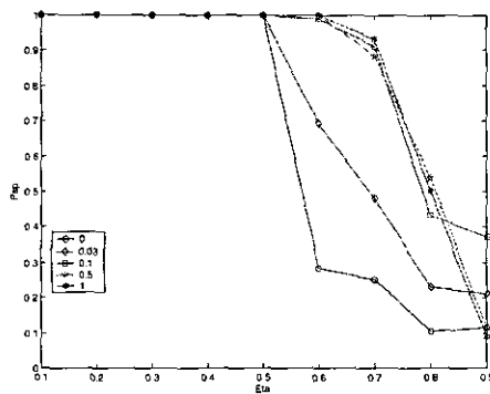
Fig. 5. P_{sp} vs. \eta in a WS small-world network at steady state
