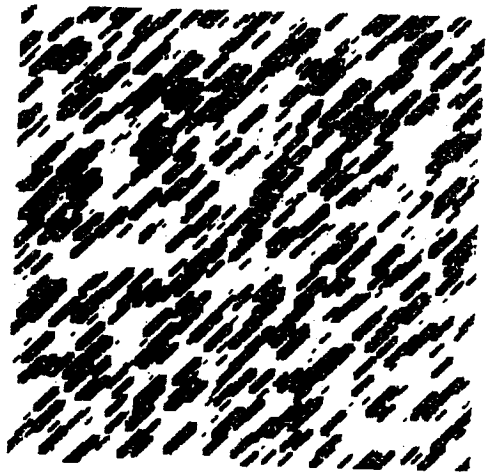
Fig. 10. Result of intersecting the DRS realization of Fig. 9 with another (independent) realization of the noise DRS N .
