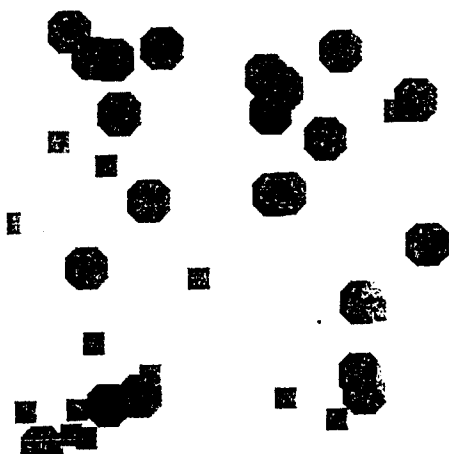
Fig. 3. Realization of the union of two DRBRs's.
