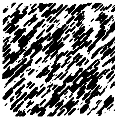
Fig. 7. Realization of the signal DRS X .
