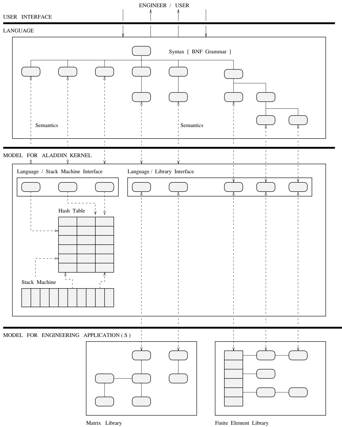
FIG. 8. : Interaction of Language and Underlying Model
