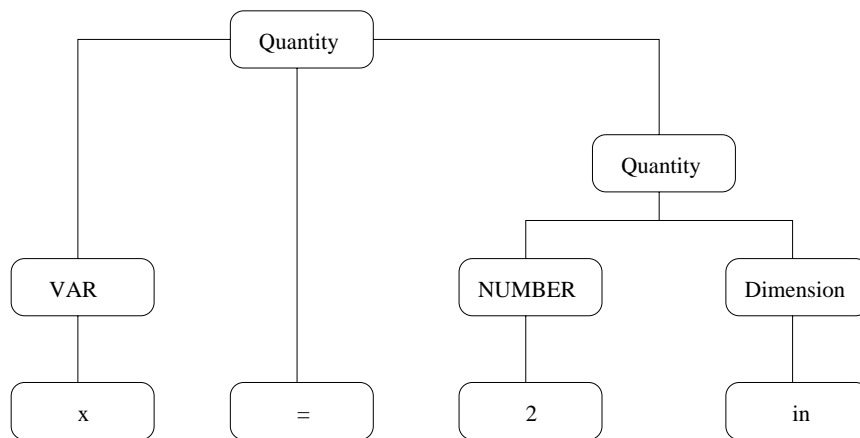
FIG. 10. : Parse tree for x = 2 \text{ in}
