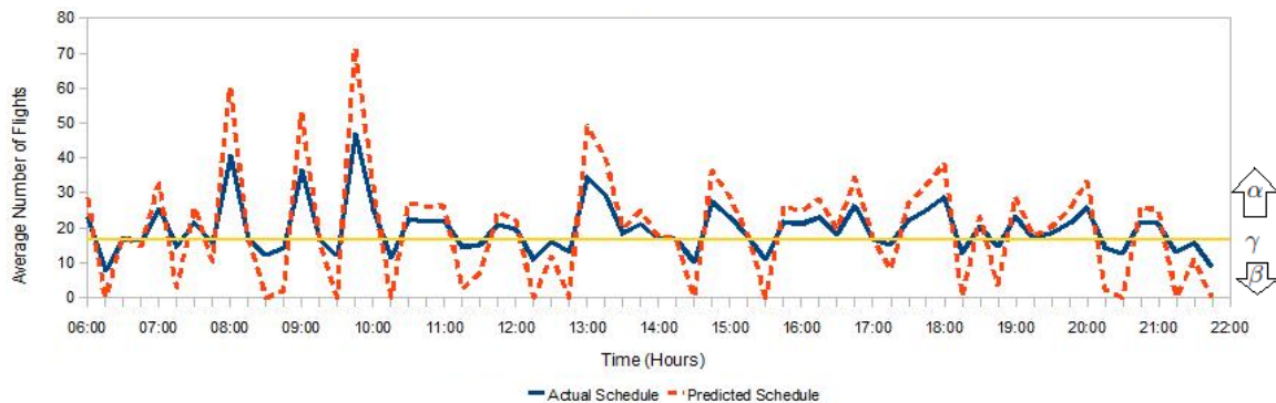
Figure 3-9: Result of schedule adjustment algorithm applied to ORD departures data for August, 2007. Actual (constrained) schedule had CVAR=0.3940 ; projected schedule had CVAR=0.8056 , which was the value estimated by the regression model.
