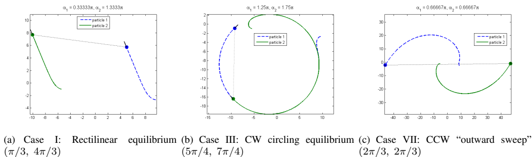
Fig. 2. These MATLAB simulations illustrate a selection of the different cases described in table I. The particular choices of (\alpha_1, \alpha_2) for each simulation are listed in the captions associated with each figure.
